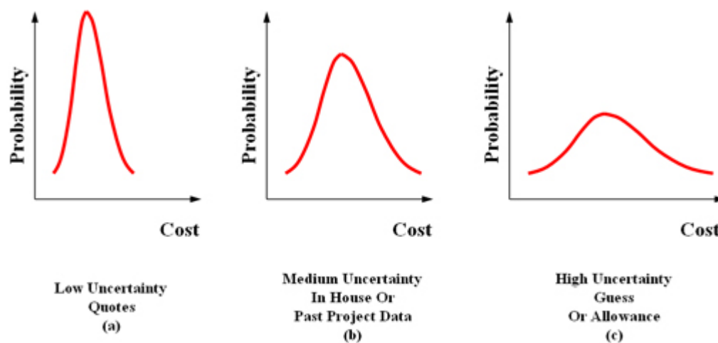
Figure 1: Probability Distribution Examples
